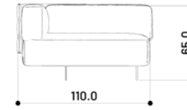
Corner Element - Front View - CCL/CCR
