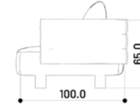
Two seater - Side view - 2S
