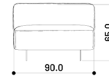
Central Element - Front View - CM
