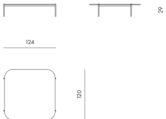
Linea H - Coffee Table Code : CT120
