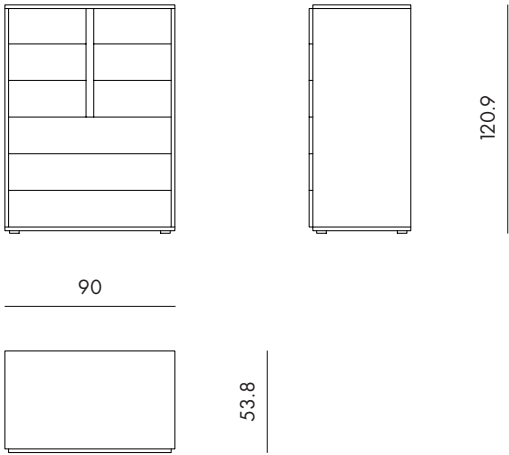
River - Tall Chest Code : TC90
