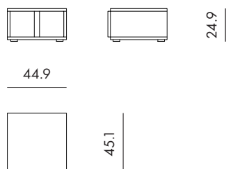
River - Night Stand Code : NST1D45
