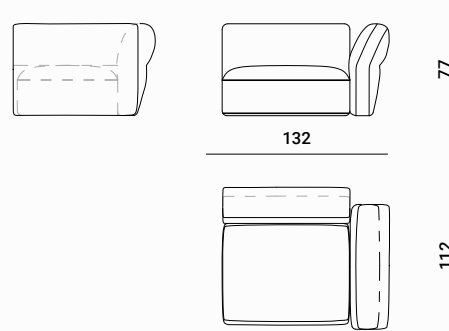
Oasi : Lateral element maxi with right armrest Code : LMR
