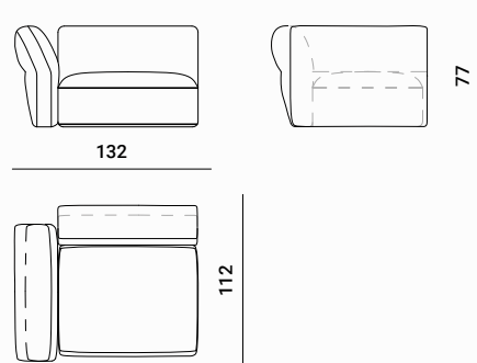
Oasi : Lateral element maxi with left armrest Code : LML
