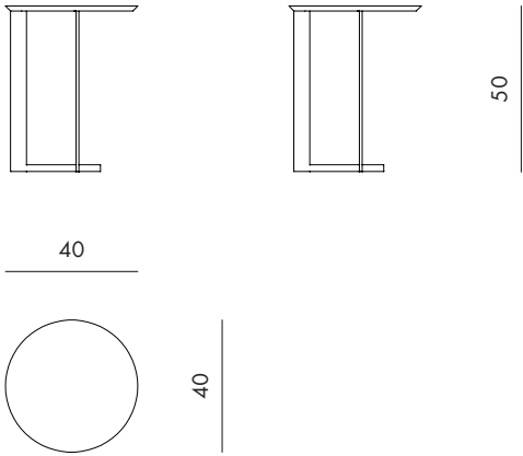
Cricket - Service Table Code : ST 40RO
