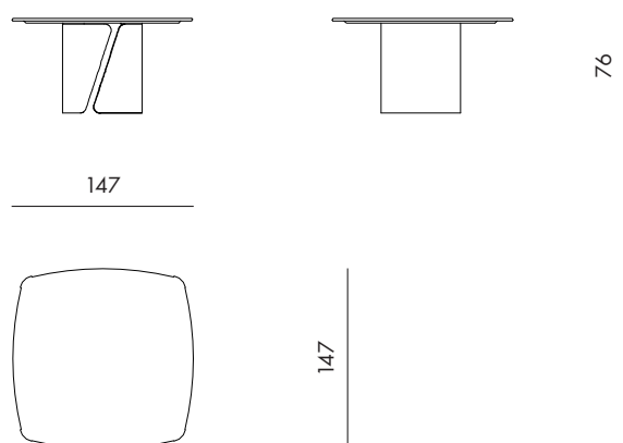
Sonic - Square Code : TAV147QS
