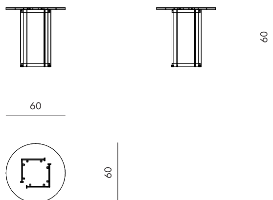
Puzzle - Service Table Code : STH 60RO
