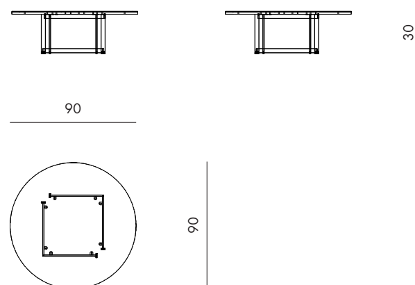
Puzzle - Coffee Table Code : CTL 90RO
