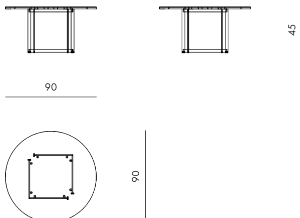
Puzzle - Coffee Table Code : CTM 90RO
